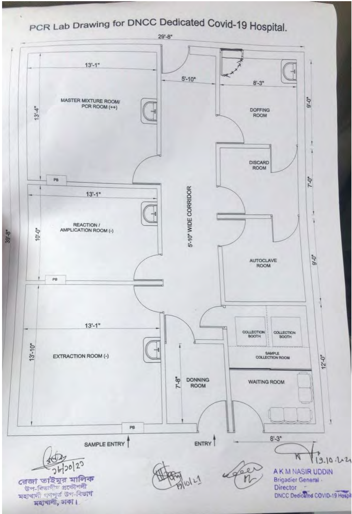
Figure: Proposed Plan for PCR Laboratory at DNCC dedicated COVID-19 Hospital
