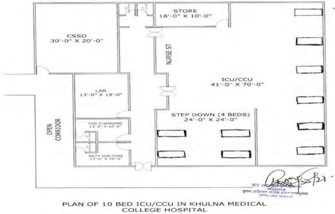
Figure: Proposed Plan for Installation of Medical Gas System (ICU) at KMCH
